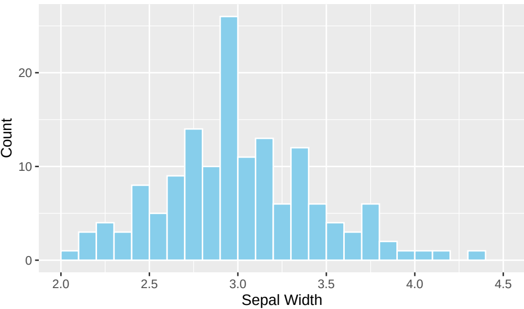
'breaks' option
