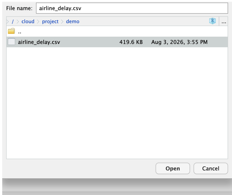
Figure 5.4: Select file
