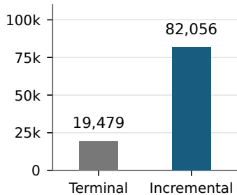
(b) Distinct letter strings
