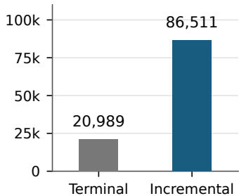
(a) Accepted token pairs
