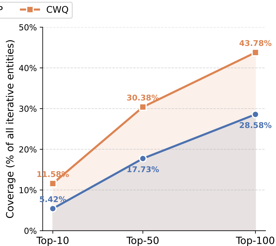
All Entities Considering Iterative Traversal
