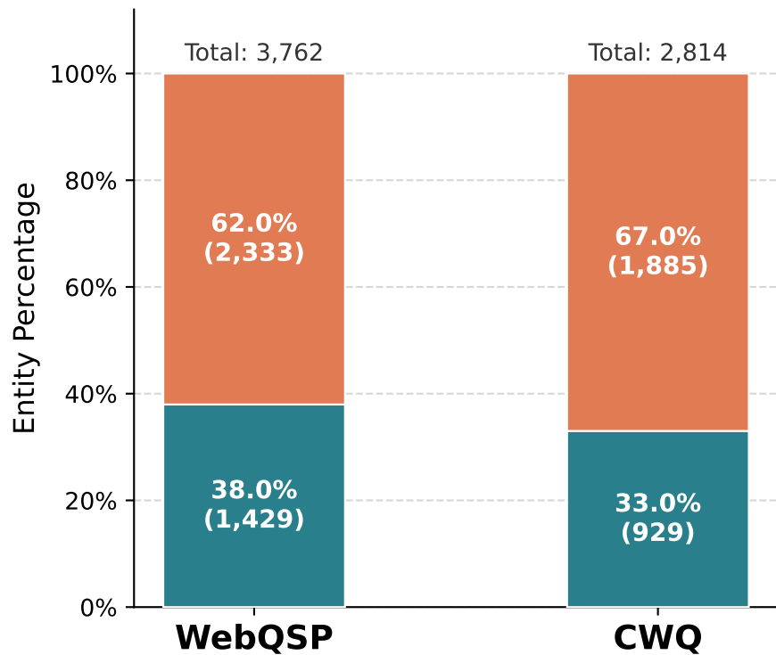
All Entities Considering Iterative Traversal
