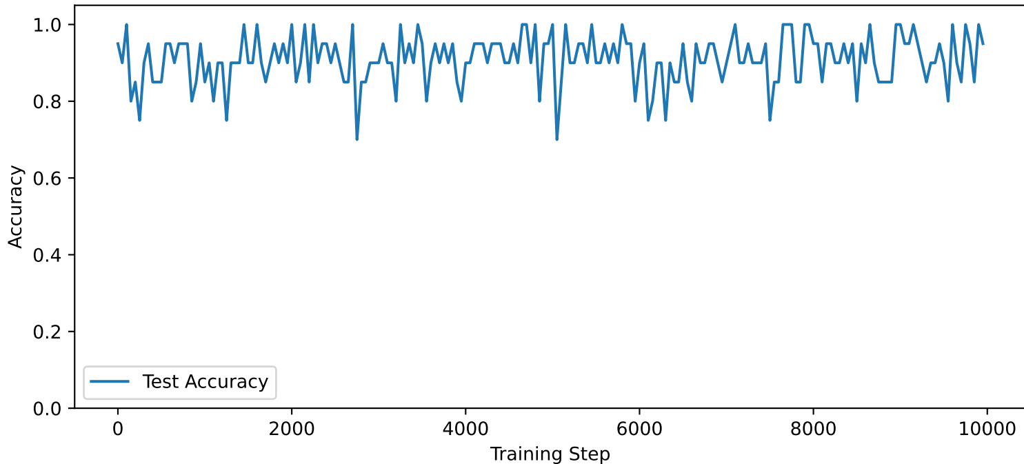
Odor Detection Accuracy Over Training, with a mean of 0.910
