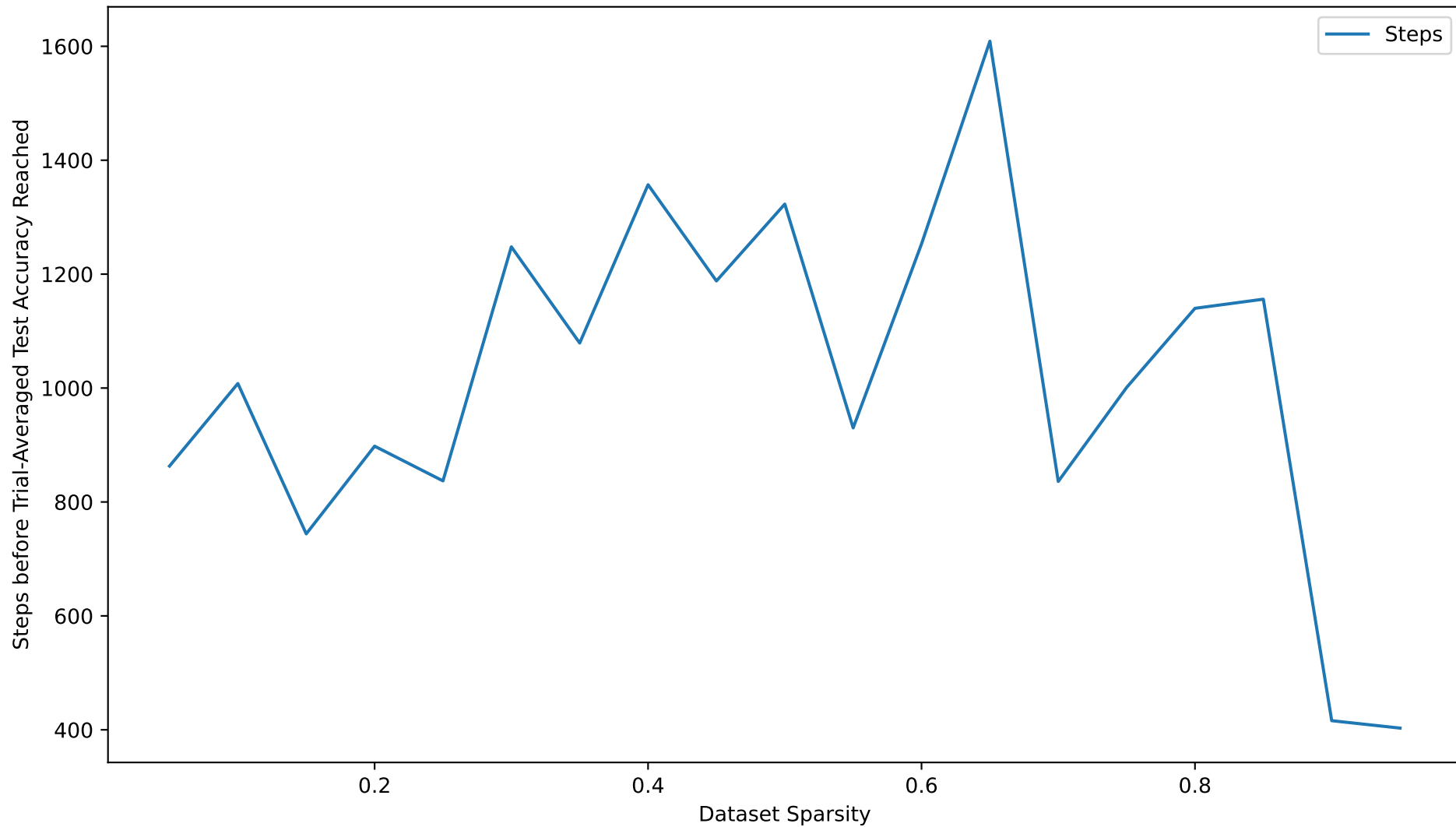
Steps before Trial-Averaged Test Accuracy of 0.95 Reached vs. Dataset Sparsity (m=50, n=100)
