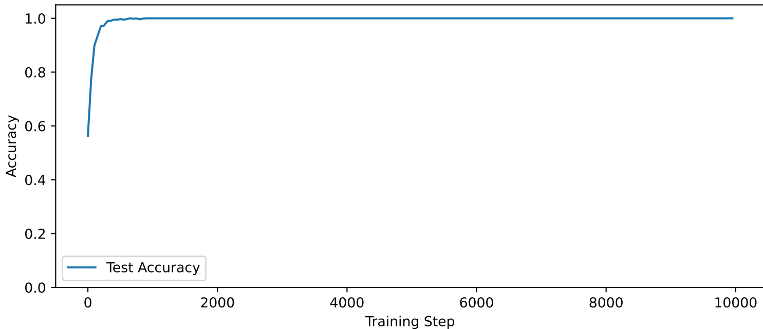
Odor Detection Accuracy Over Training with Sparsity=0.9, with a mean of 1.000 90% Mean Accuracy Achieved at Step 10
