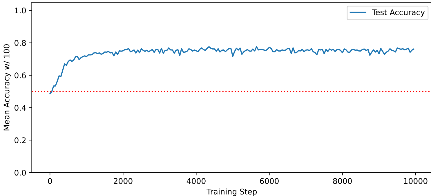
Odor Detection Accuracy Over Training, with a mean of 0.753
