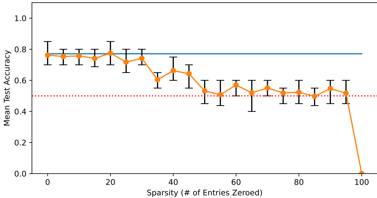
Mean Accuracy vs. Sparsity over 100 Iterations with m=100 , n=50 (25% and 75% Quantile Errorb
