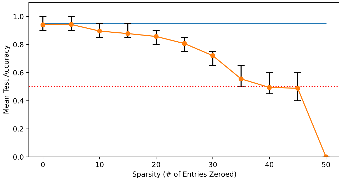
Mean Accuracy vs. Sparsity over 100 Iterations w/ m=50 , n=100 (25% & 75% Quantile Errorbar)
