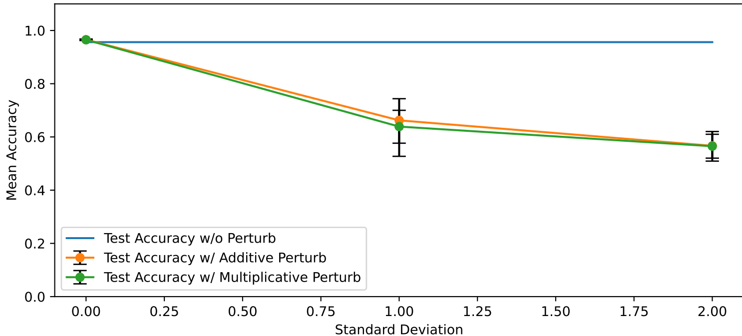
Mean Accuracy vs. Standard Deviation (25% and 75% Quantile Bars)
