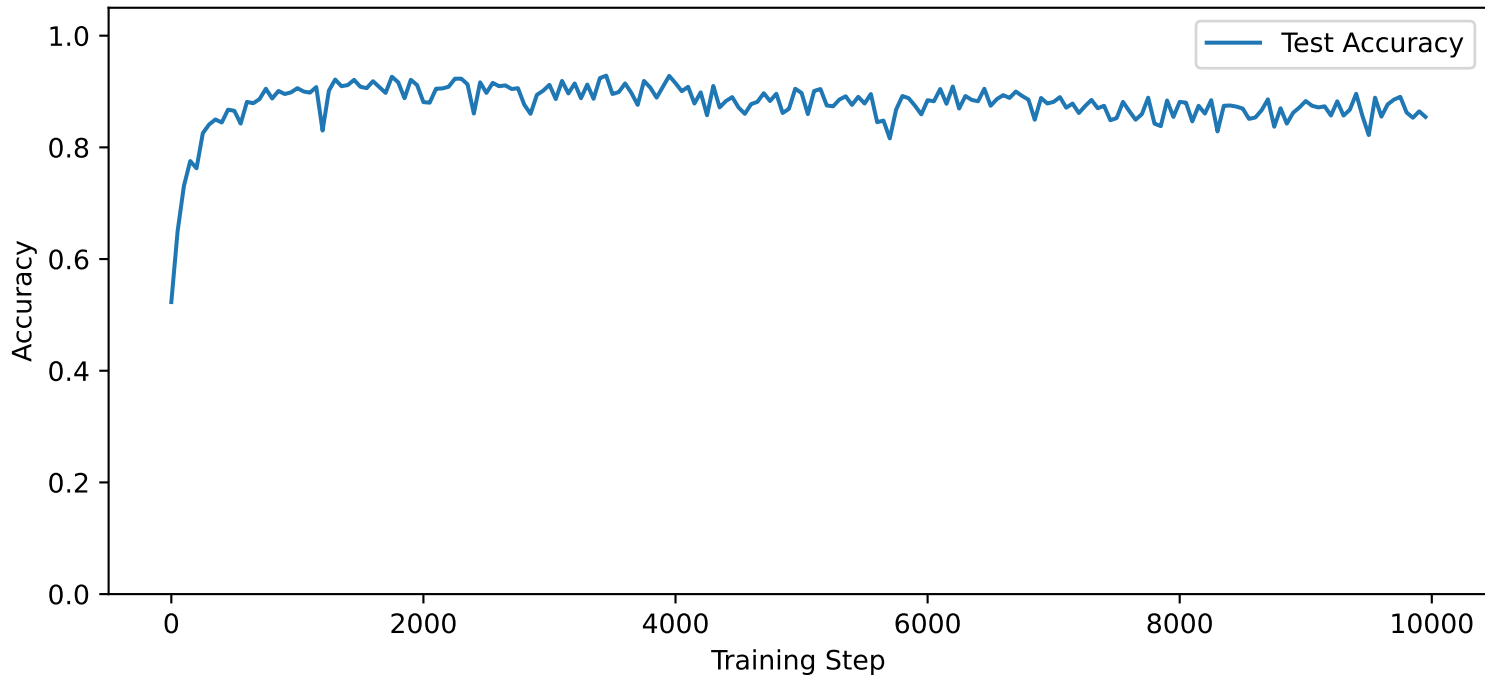
Odor Detection Accuracy Over Training, with a mean of 0.873
