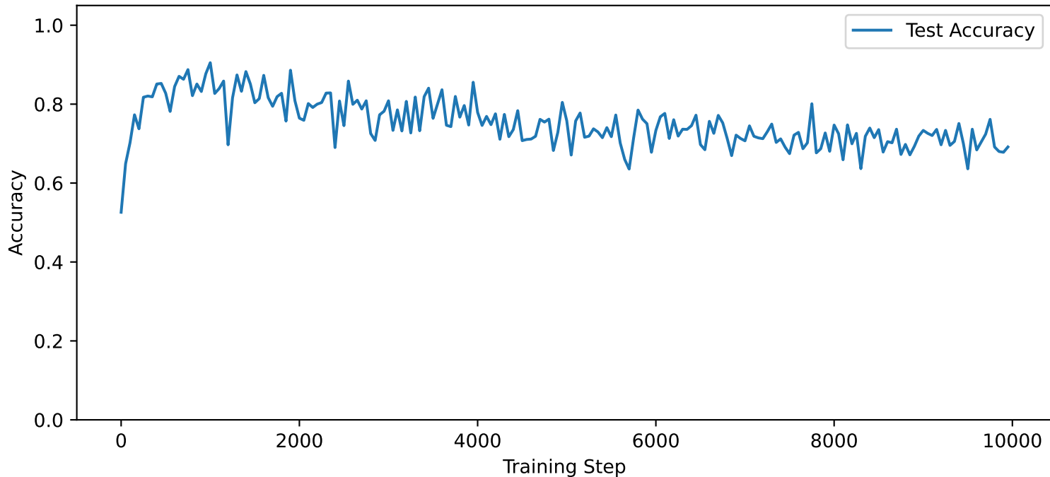
Odor Detection Accuracy Over Training, with a mean of 0.718
