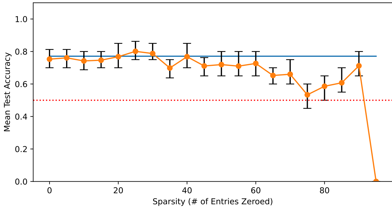
Mean Accuracy vs. Sparsity over 100 Iterations w/ m=100 , n=50 (25% & 75% Quantile Errorbar)
