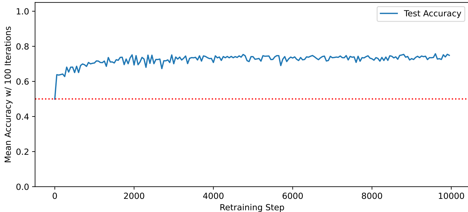
Odor Detection Accuracy Over 10000 Retraining Steps, with a mean of 0.735
