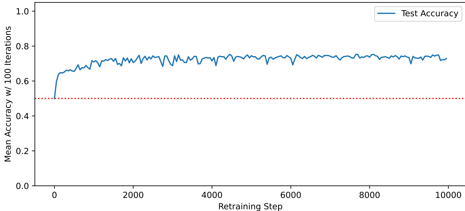
Odor Detection Accuracy Over 10000 Retraining Steps, with a mean of 0.737
