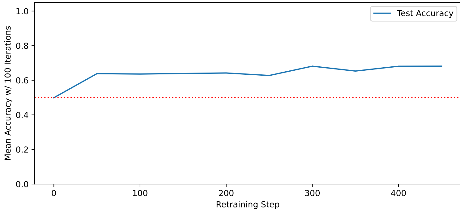
Odor Detection Accuracy Over 500 Retraining Steps, with a mean of 0.661
