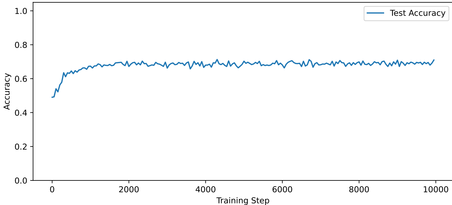
Odor Detection Accuracy Over Training, with a mean of 0.689
