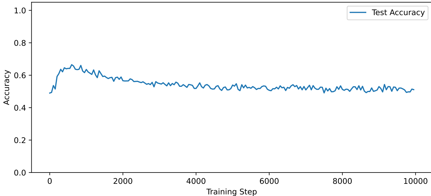
Odor Detection Accuracy Over Training, with a mean of 0.518
