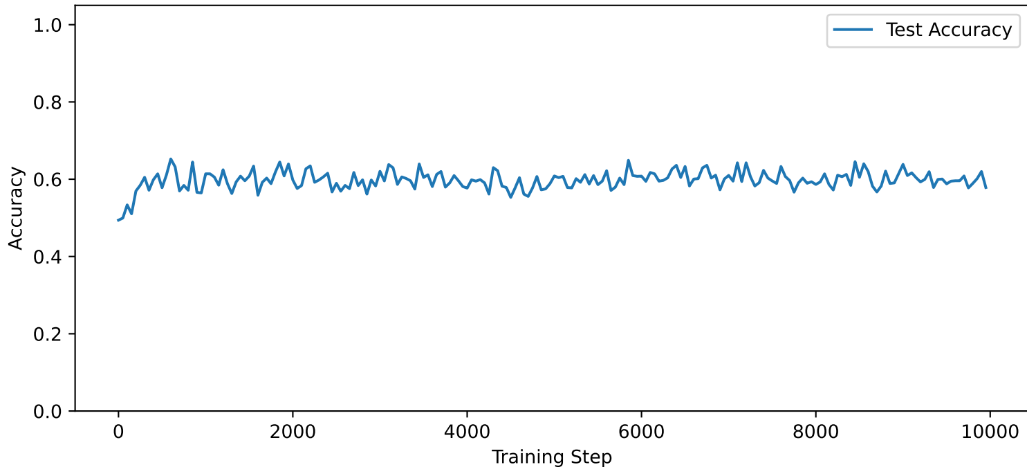
Odor Detection Accuracy Over Training, with a mean of 0.603
