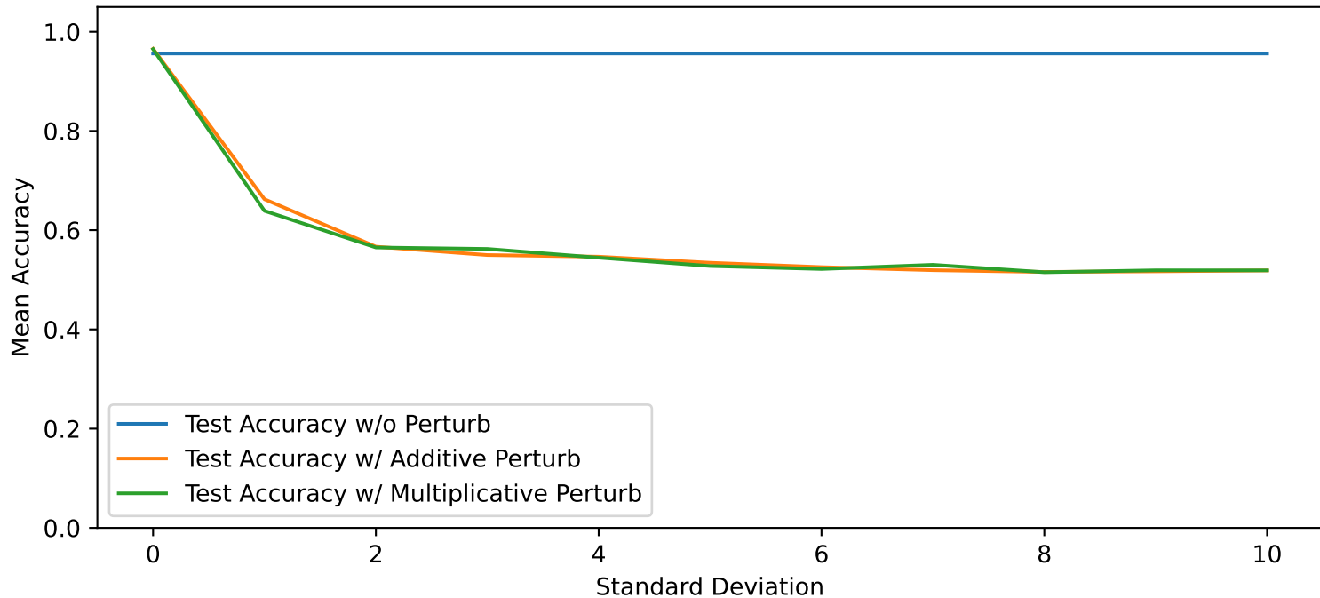
Mean Accuracy vs. Standard Deviation
