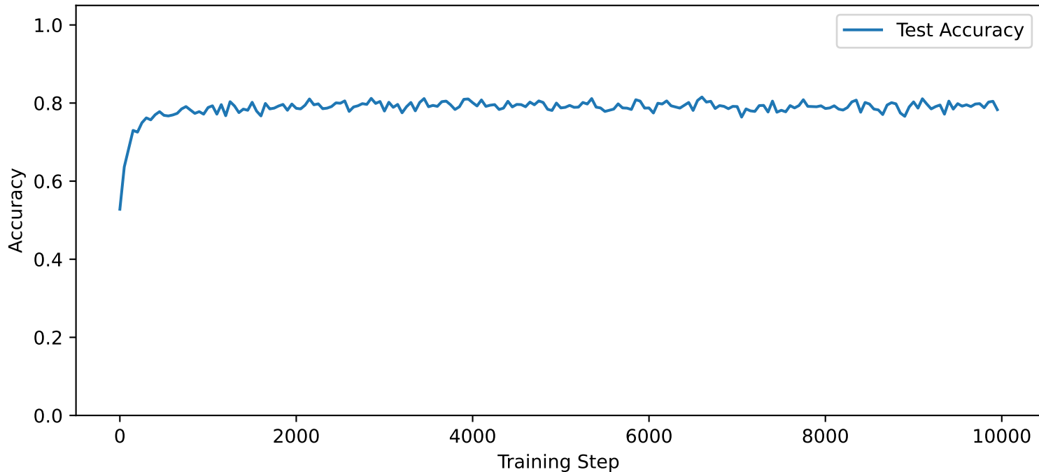
Odor Detection Accuracy Over Training, with a mean of 0.791
