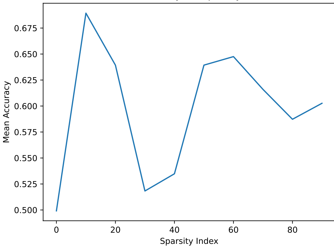
Mean Accuracy vs. Sparsity Index
