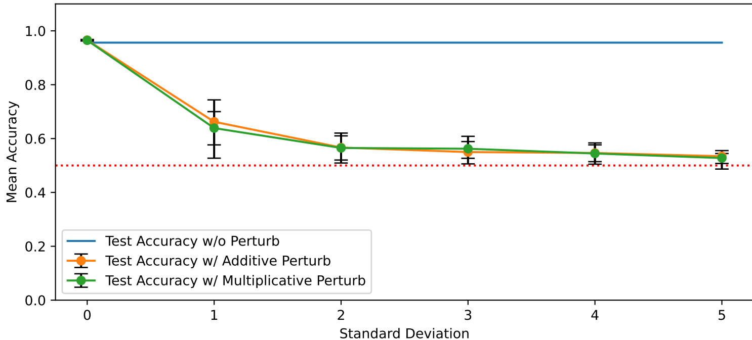
Mean Accuracy vs. Standard Deviation (25% and 75% Quantile Bars), m=50 , n=100
