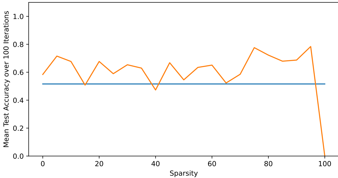
Mean Accuracy vs. Sparsity
