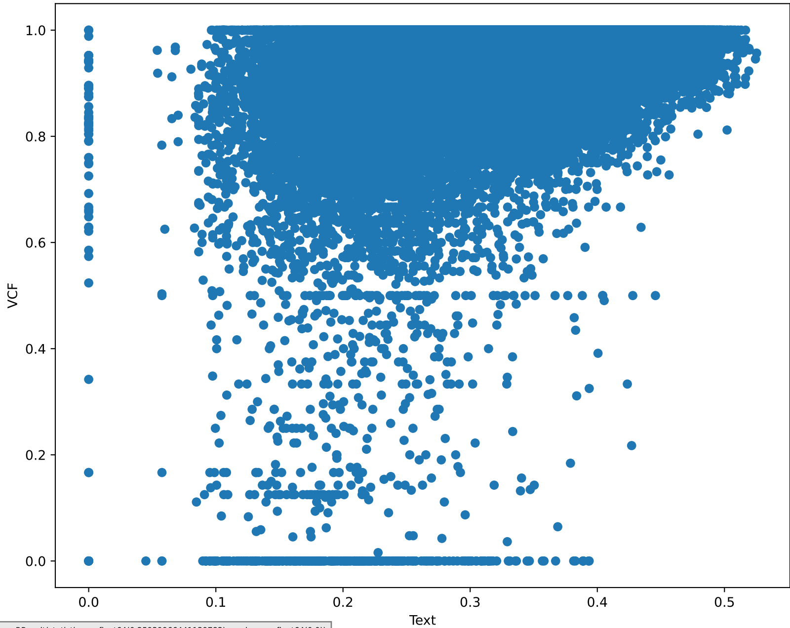
Itemwise RSA Scatter Plot w/ Threshold = 10
