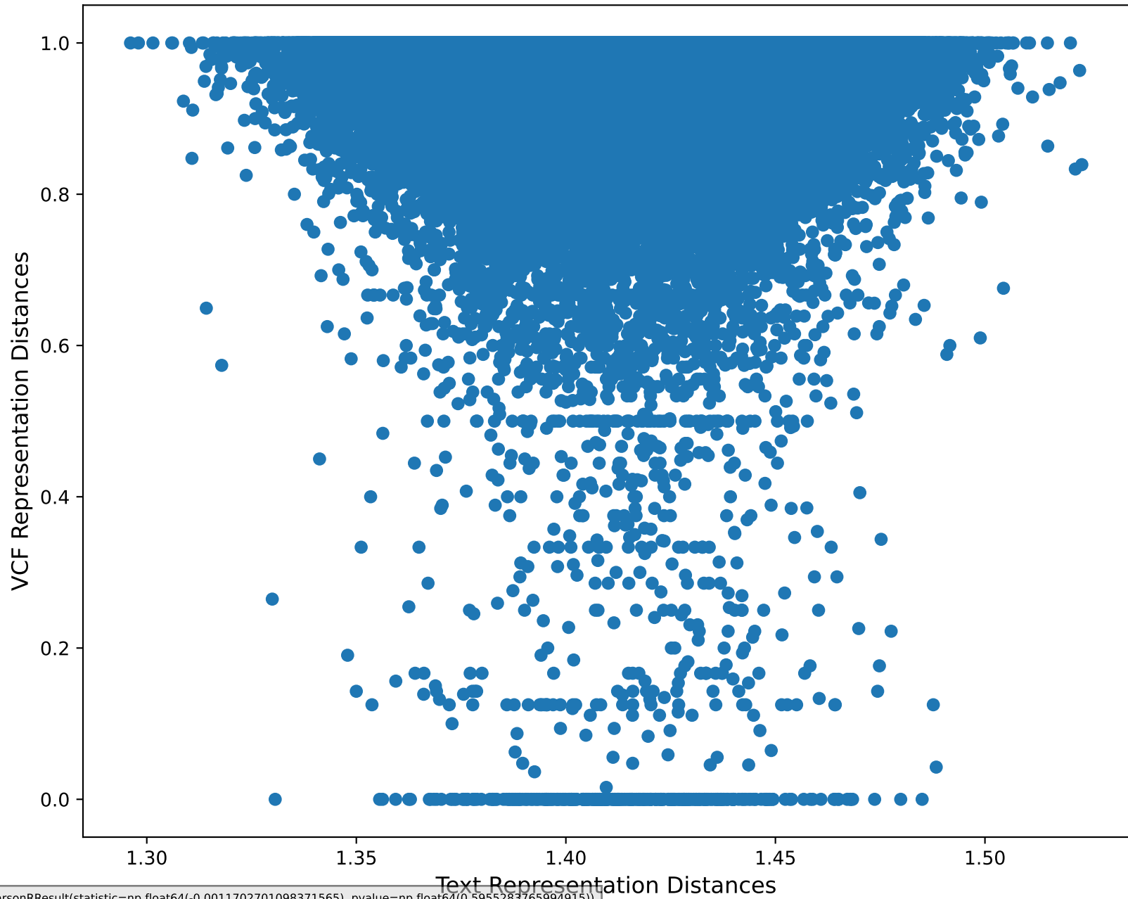
Random Embedding Itemwise RSA Scatter Plot w/ Threshold = 10
