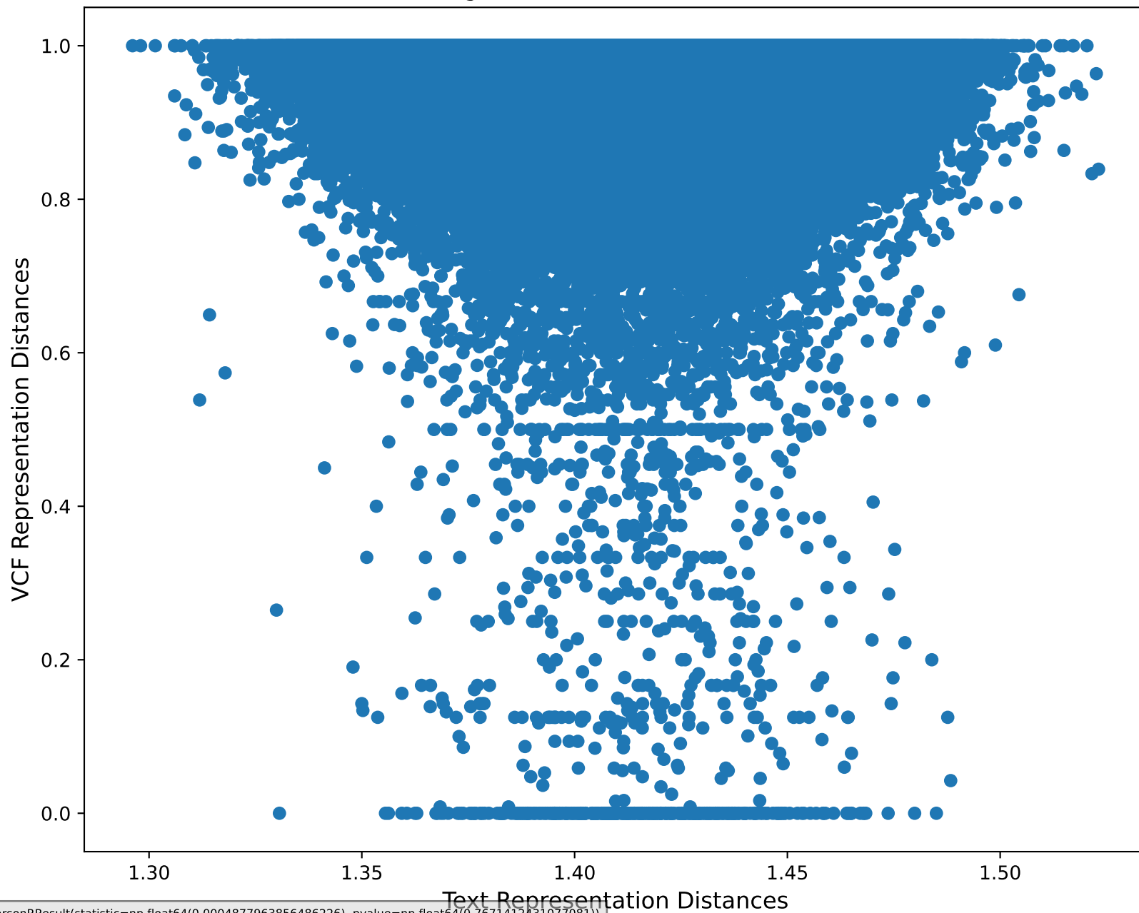
Random Embedding Itemwise RSA Scatter Plot w/ Threshold = 5
