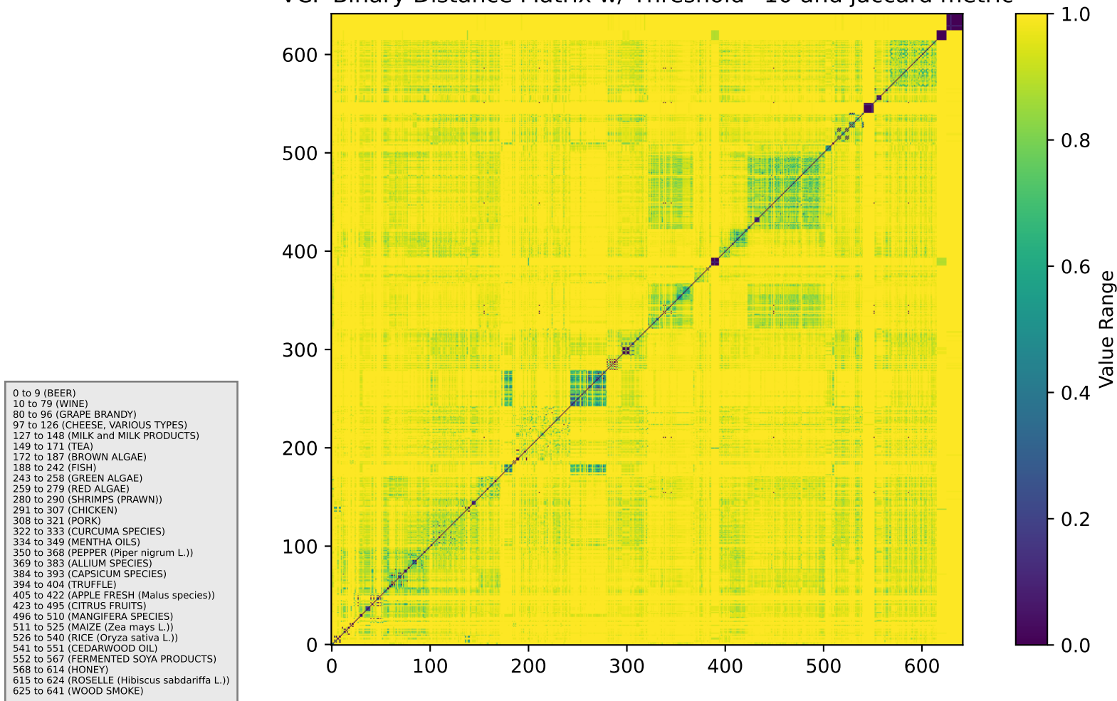
VCF Binary Distance Matrix w/ Threshold=10 and jaccard metric
