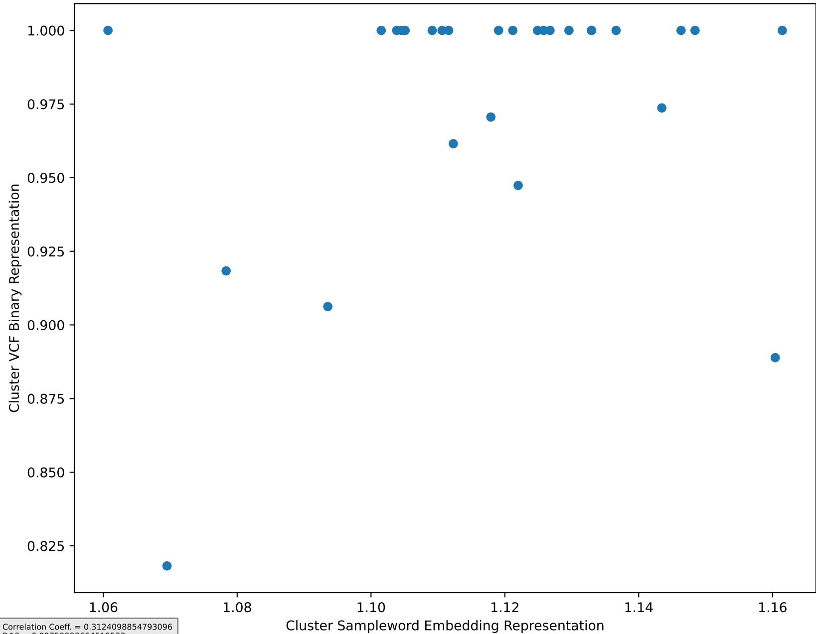
Scatter Plot with X: sample word representation, Y: VCF binary representation
