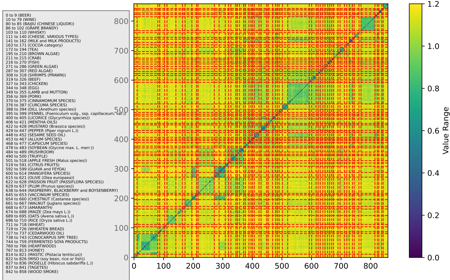
Itemwise Distance Matrix on Text Dataset w/ Threshold=5 and Euclidean Metric
