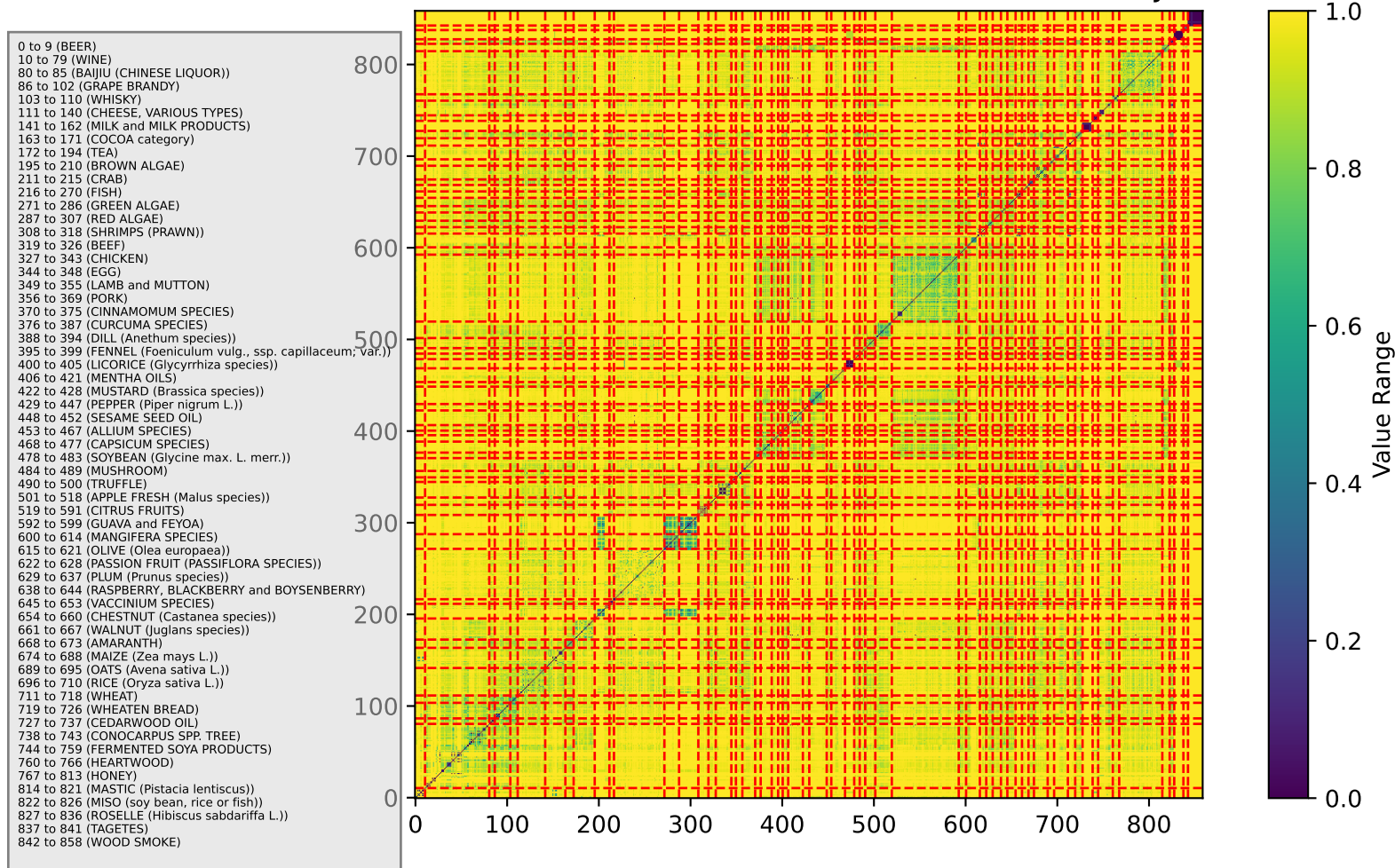
Itemwise Distance Matrix on VCF Dataset w/ Threshold=5 and Jaccard Metric
