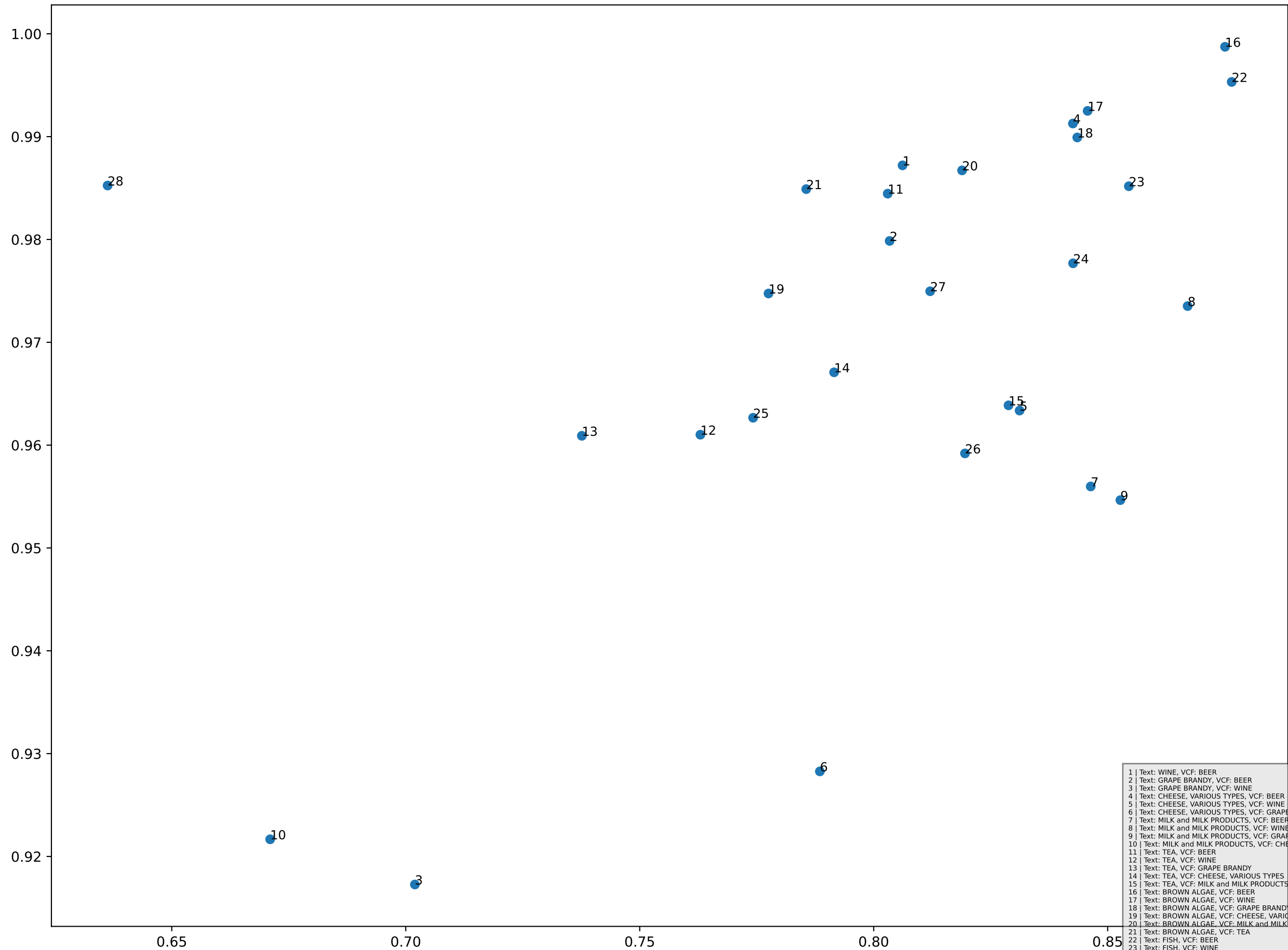
Clusterwise RSA Scatter Plot w/ Threshold = 10
