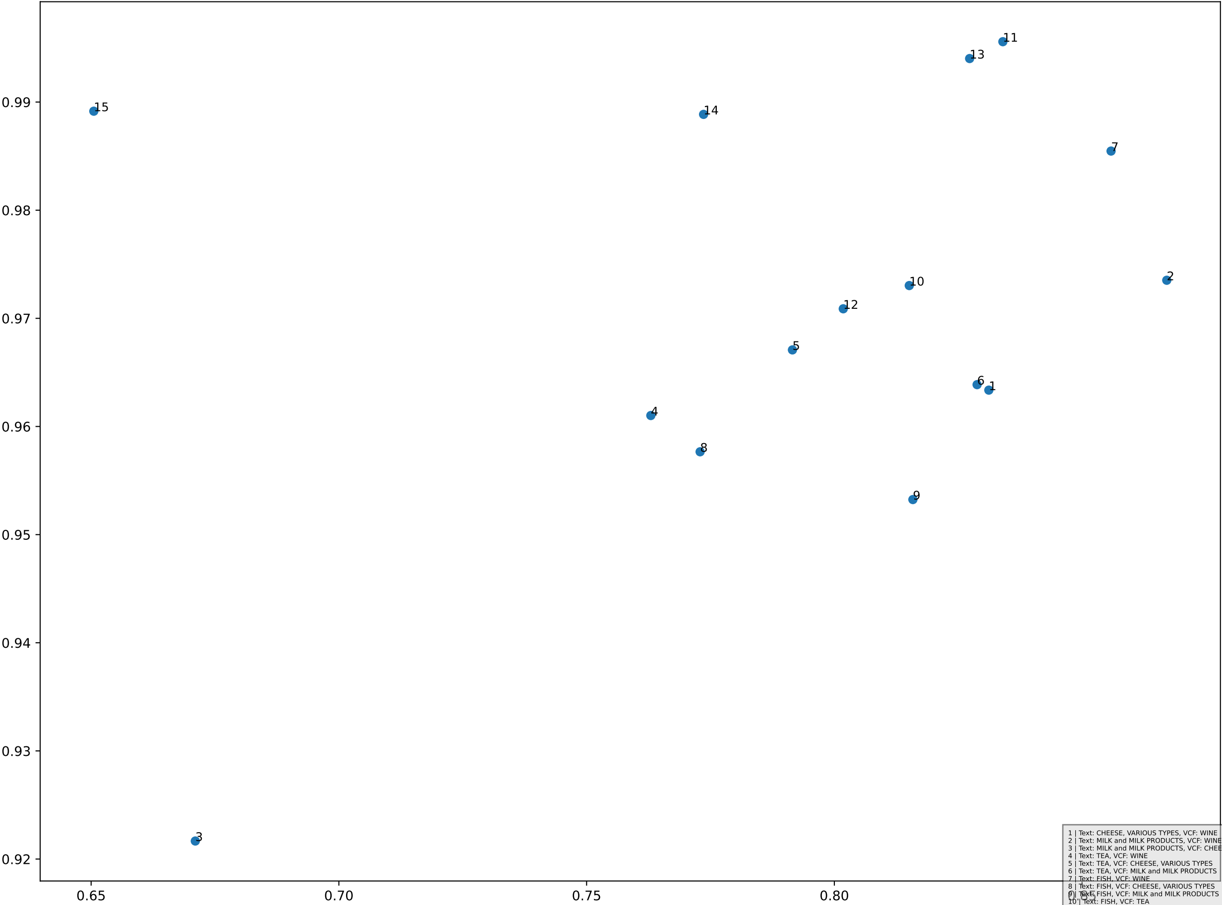
Clusterwise RSA Scatter Plot w/ Threshold = 20
