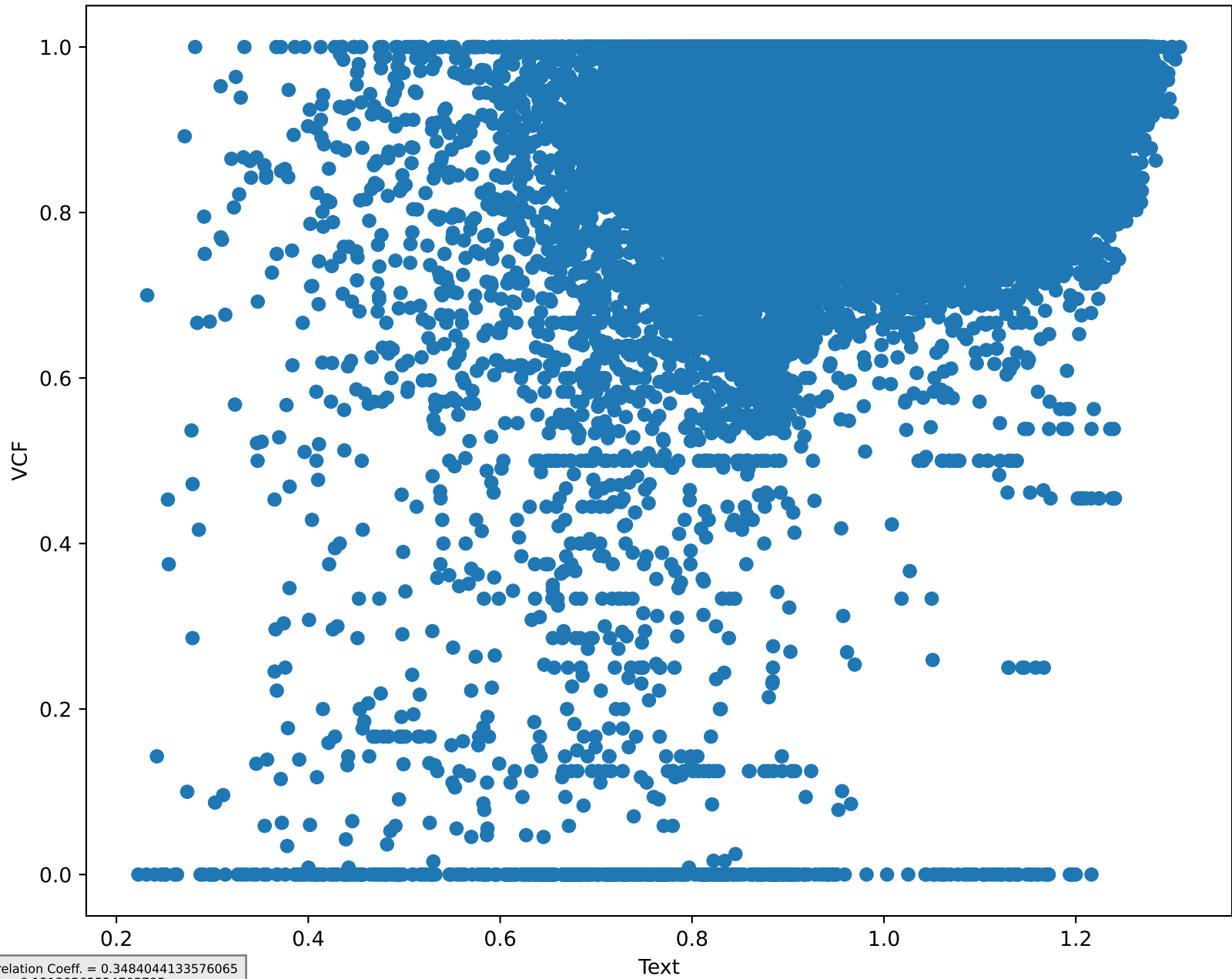
Itemwise RSA Scatter Plot w/ Threshold = 5
