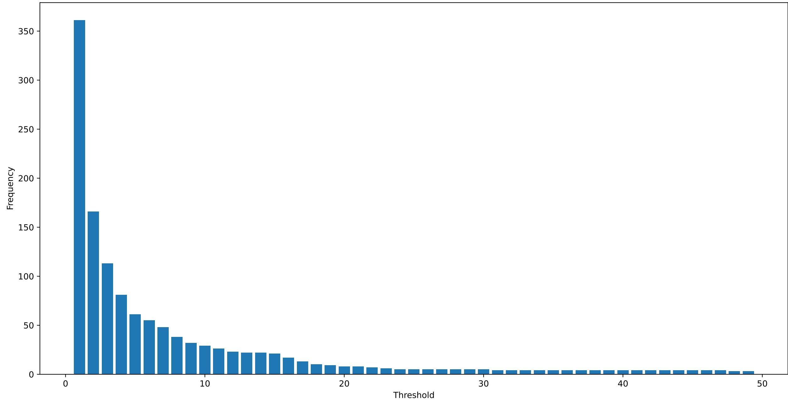
Frequencies vs. Sample Count Threshold
