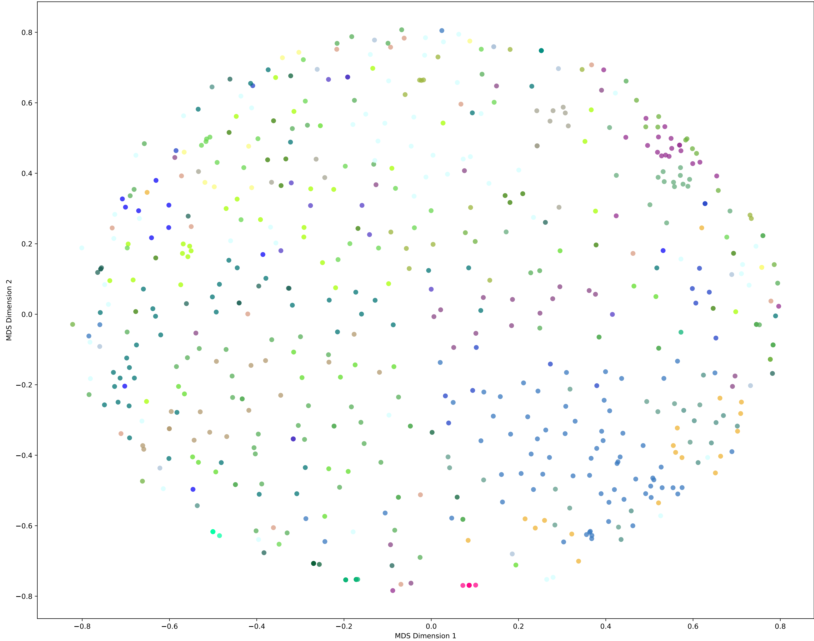
MDS with 2 Dimensions on VCF Dataset with jaccard Metric & Threshold = 10
