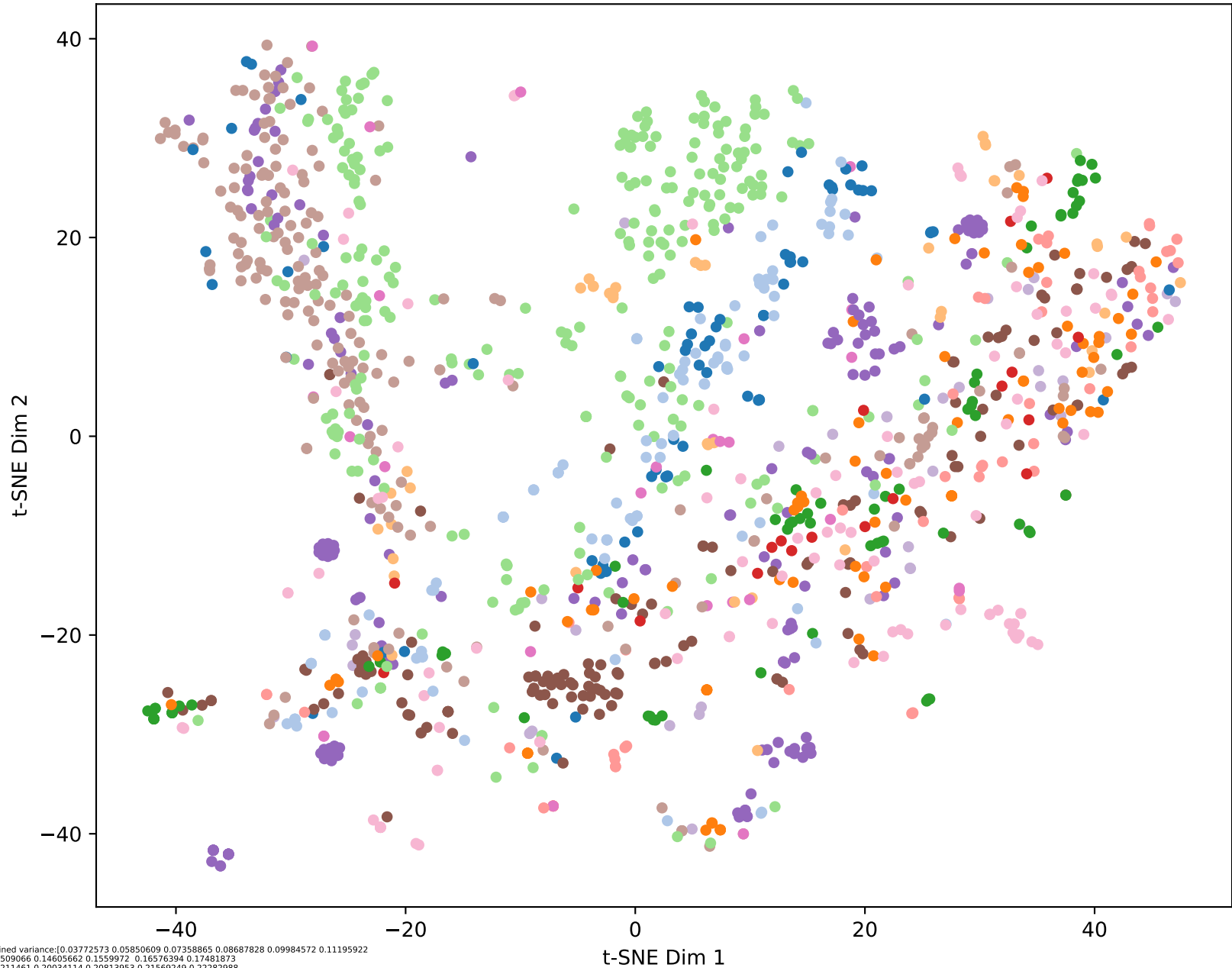
2D t-SNE of Dataset PCA-Reduced to 50 Components (Color by Food Class)
