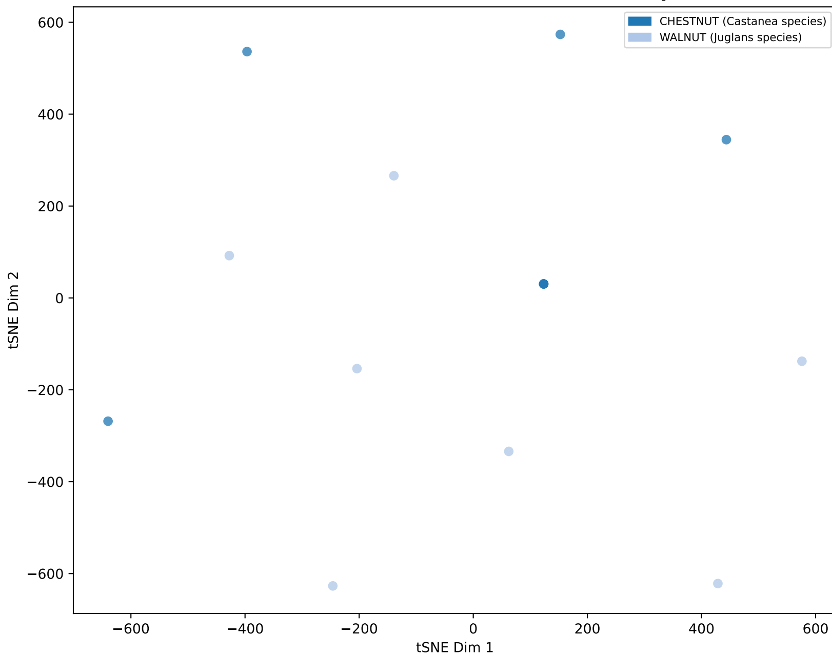
2D t-SNE of NUTS PCA-Reduced to 10 Components (Color by Food Type) Cumulative explained variance:[0.32202363 0.48752991 0.61811902 0.72886861 0.81917838 0.90112667 0.94213896 0.97133967 0.98755431 0.99652384]
