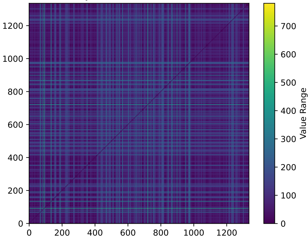
PCA-Reduced VCF Binary Data Correlation Matrix w/ euclidean metric
