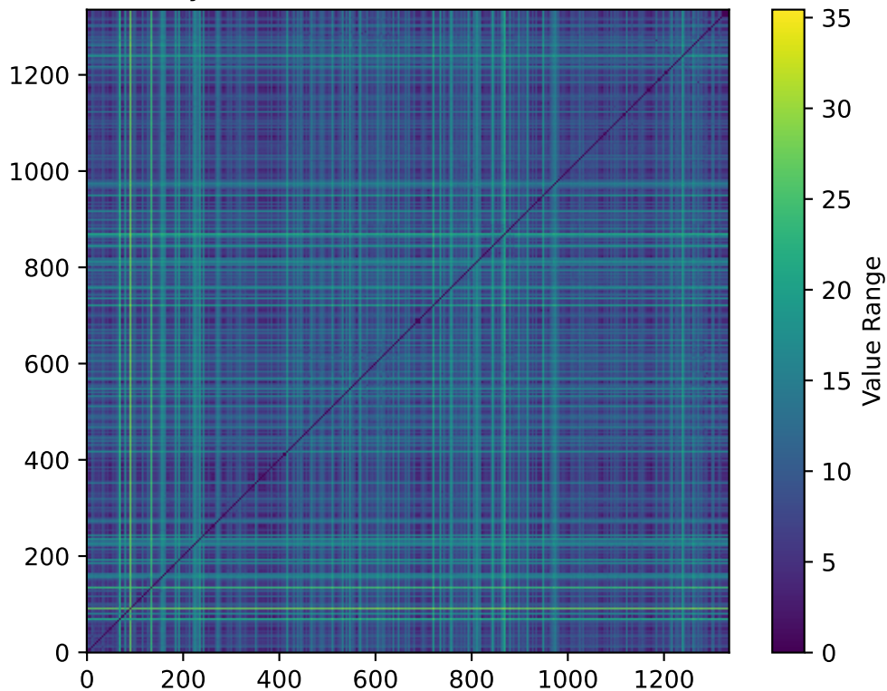
VCF Binary Correlation Matrix w/ euclidean metric
