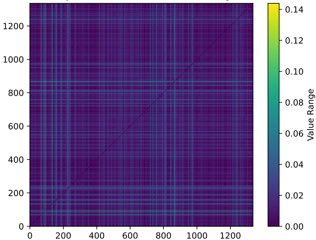
VCF Binary Correlation Matrix w/ hamming metric
