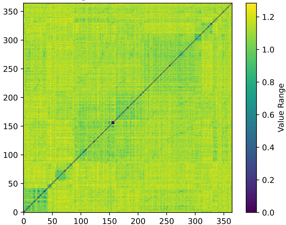
Food Word Embeddings Correlation Matrix w/ euclidean metric
