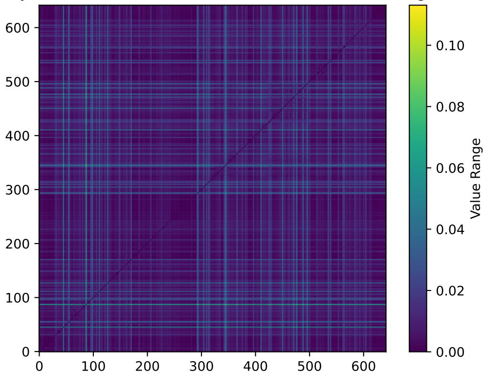
VCF Binary Correlation Matrix w/ Threshold=10 and hamming metric
