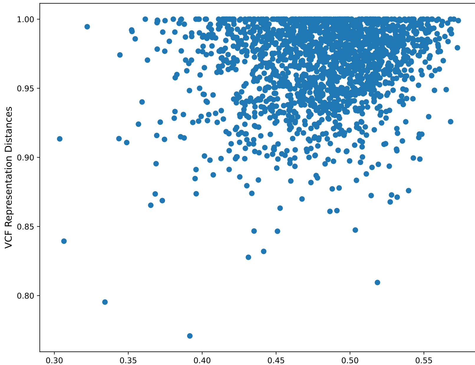
Clusterwise RSA Scatter Plot w/ Threshold = 5
