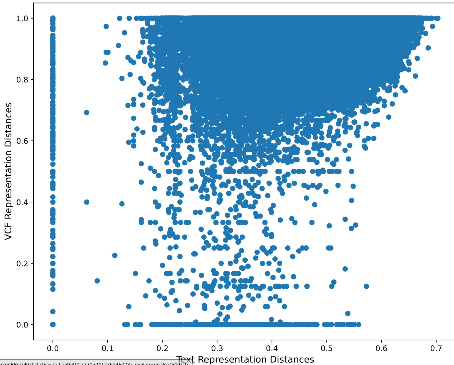
Itemwise RSA Scatter Plot w/ Threshold = 5
