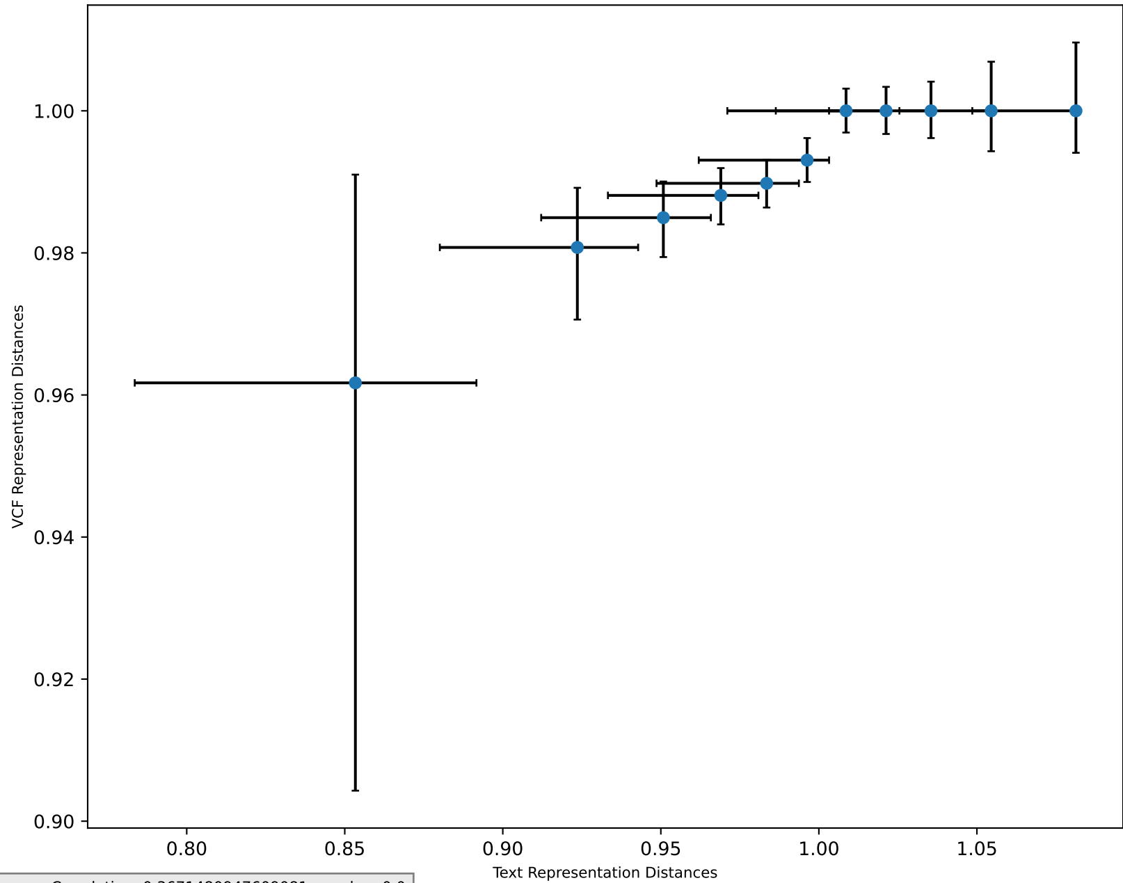
Raw Word Itemwise RSA Scatterplot w/ Threshold=5
