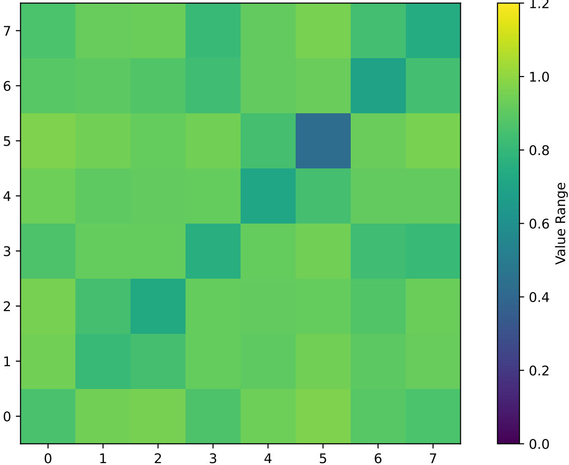
Clusterwise Distance Matrix w/ Threshold=20 and Euclidean Metric
