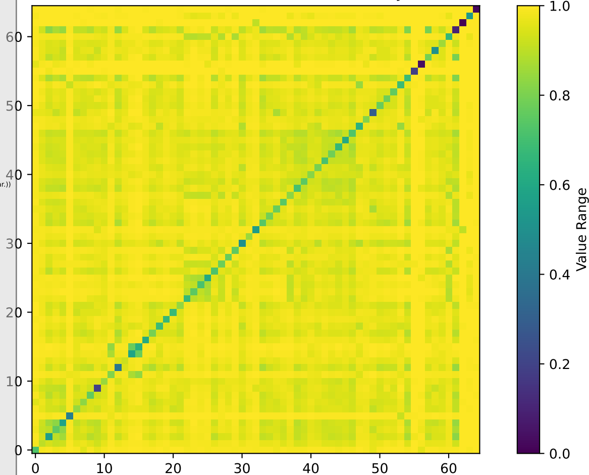
Clusterwise Distance Matrix w/ Threshold=5 and Jaccard Metric
